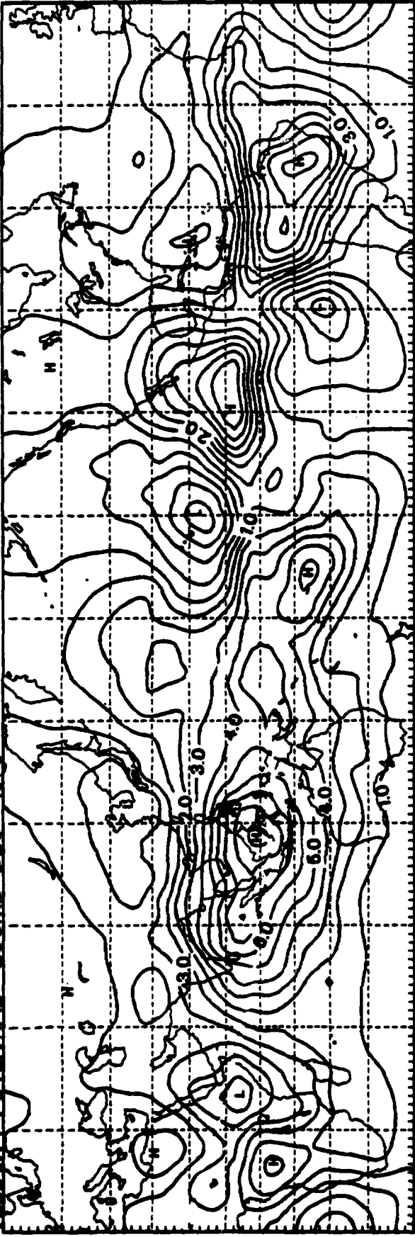
VELOCITY POTENTIAL 200MB DEC 1976
